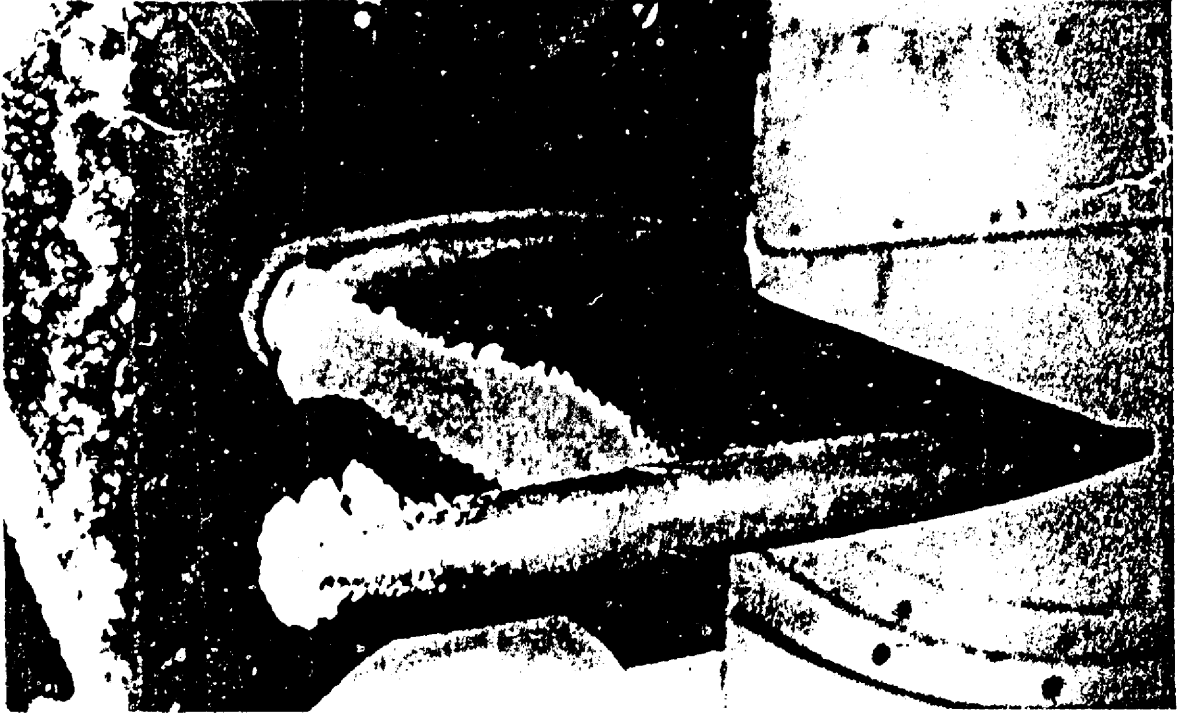
FIGURE 94. External icing on a pitot tube.
