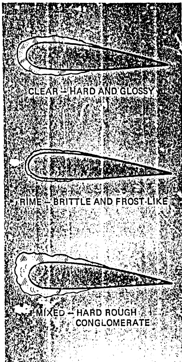
FIGURE 90. Clear, rime, and mixed icing on airfoils.
