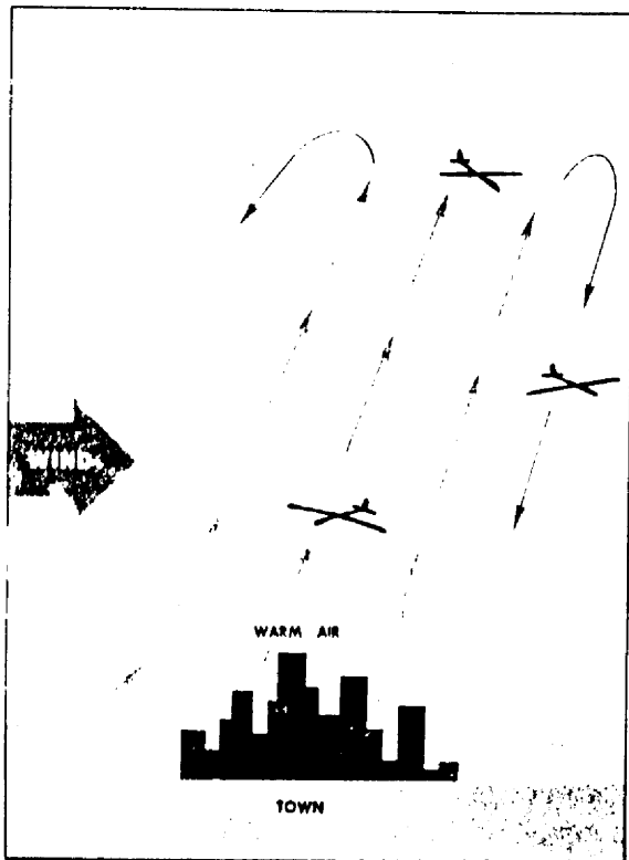
FIGURE 156. Wind causes thermals to lean. A pilot seeking lift beneath soaring birds, other aircraft, or cumulus clouds should enter the thermal upwind from the higher level visual cue.
