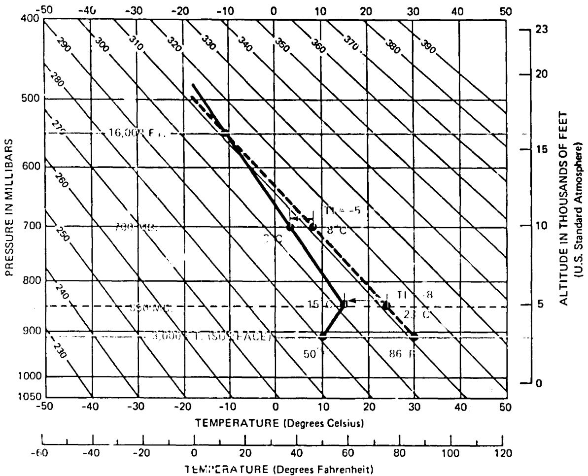
FIGURE 163. Another example of computing T's and maximum height of thermals. See discussion in caption of figure 162. By the time of maximum heating, excellent lift should be available in lower levels and moderate lift above 10,000 feet. Although thermals should continue to 16,000 feet, you could expect weak lift above 12,000 or 13,000 feet because of the small difference between temperatures in the thermal and in the surrounding air.
